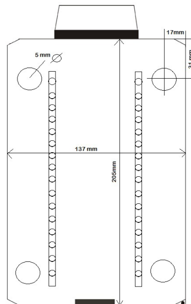
Rear of alarm for mounting dimensions.
